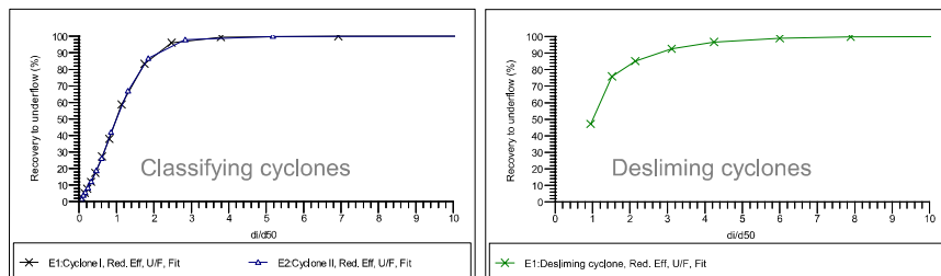
Figure 4. Fitted Reduced Efficiency curves fitted for the third survey.
